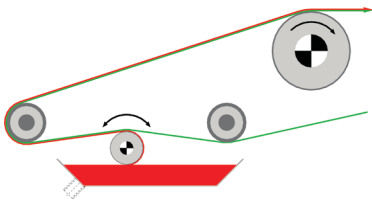
Micro Roller system
